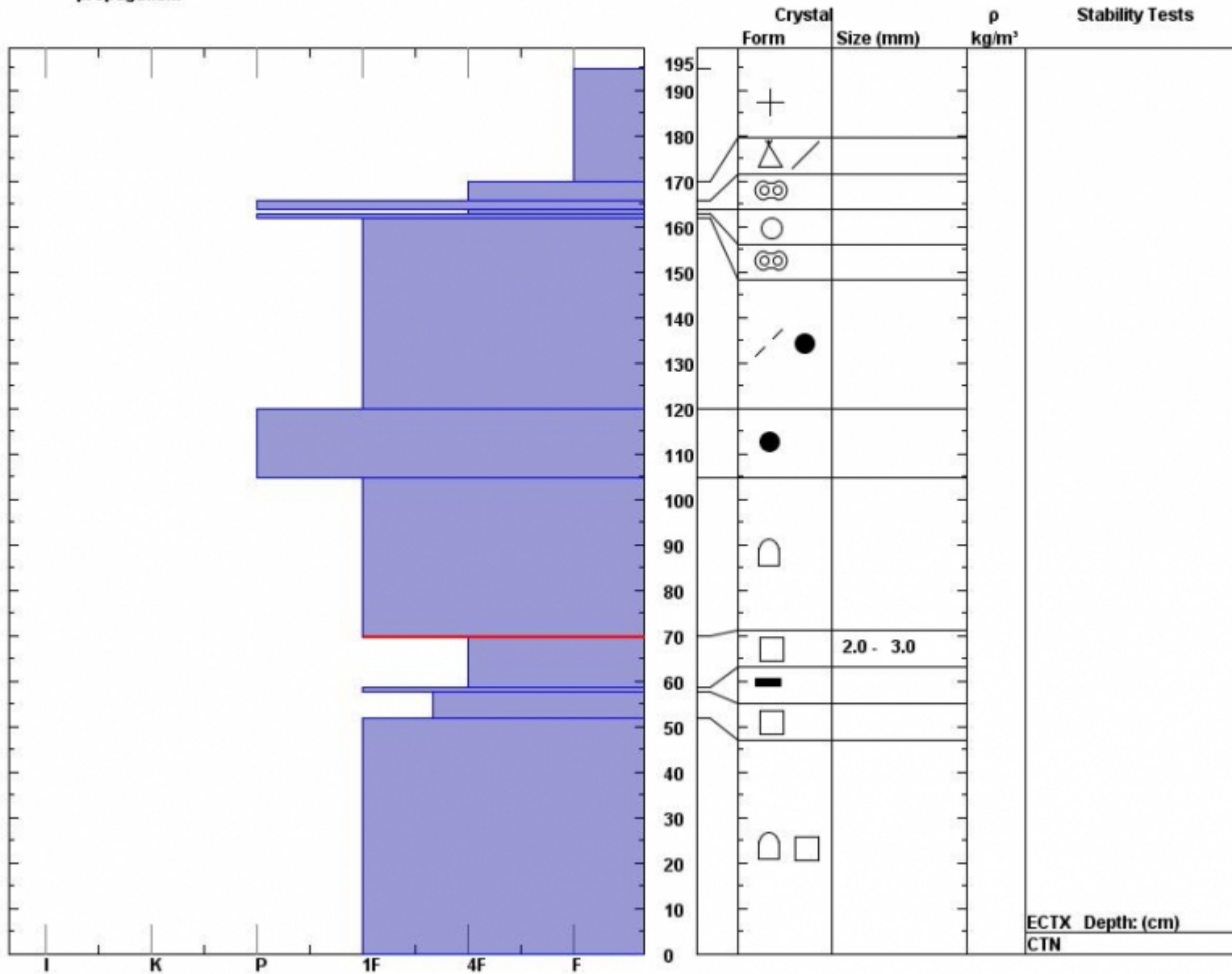
Snowpit-crown profile from natural avalanche in the Northern Bridgers on 18 March 2011
